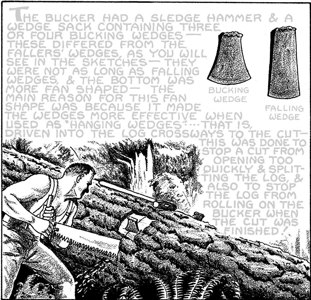
Figure 40—A bucking wedge being used as a hanging wedge. The wedge kept the cut from opening too quickly and splitting the log, and also stopped the log from rolling on the bucker when the cut was finished.—Now You're Logging, by Bus Griffiths, with permission of Harbour Publishing, Madeira Park, BC, Canada
